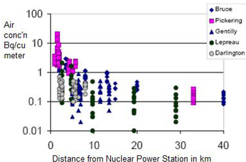
Figure 1 Annual averages of tritium concentrations in air measured at distances from nuclear power stations in Canada, 1985-1999. Abstracted from: Tritium in the Canadian Environment: Levels and Health Effects. Report RSP-0153-1 (2003). Prepared for the Canadian Nuclear Safety Commission under CNSC contract no. 87055-01-0184 by Ranasara Consultants and Richard Osborne. Data from Health Canada: Environmental Radioactivity in Canada. Radiological Monitoring Report. Ottawa, Canada: Government of Canada; 2001.
