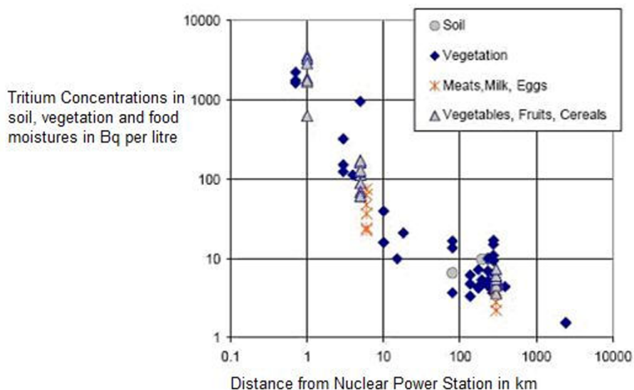
Figure 2 Tritium concentrations in vegetation/food moisture near Canadian nuclear power stations. Abstracted from: Tritium in the Canadian Environment: Levels and Health Effects. Report RSP-0153-1 (2003). Prepared for the Canadian Nuclear Safety Commission under CNSC contract no. 87055-01-0184 by Ranasara Consultants and Richard Osborne. Data from Health Canada: Environmental Radioactivity in Canada. Radiological Monitoring Report. Ottawa, Canada: Government of Canada; 2001.
